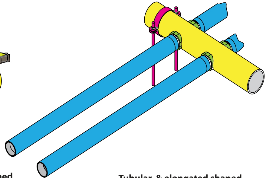
- Tubular, & elongated shaped membranes – Tubular Diffusers
